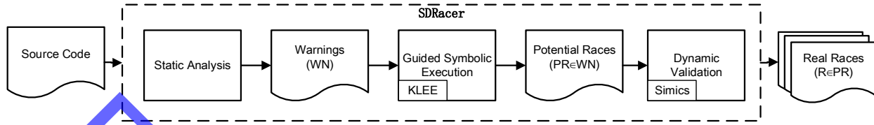
Figure 2: Overview of SDRacer framework.
