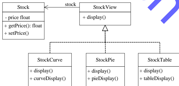
Fig.10 Business logic models
